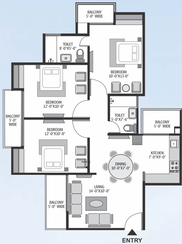
TYPE D1 - 3BHK/ 2T AREA - 1340 SQ. FT.
